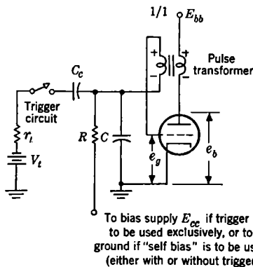
Fig. 14.15.—Circuit of a typical regenerative pulse generator.
